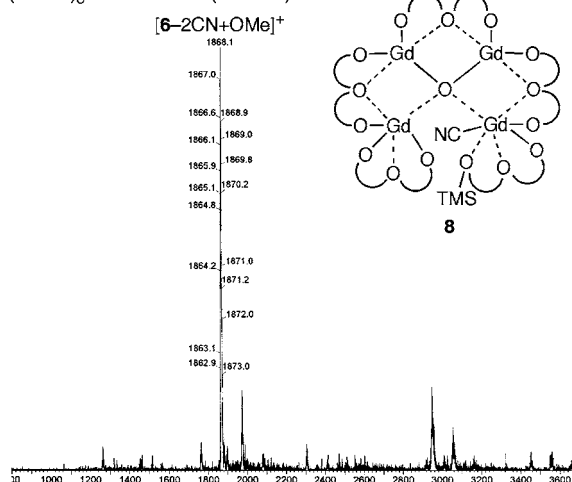
Figure 3. ESI-MS observations of the catalyst complexes.
