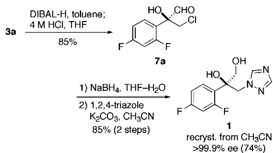
Scheme 2. Conversion to Intermediate 1
