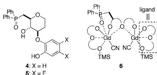
Figure 2. Chiral ligands and proposed catalyst structure for cyanosilylation of ketones.
