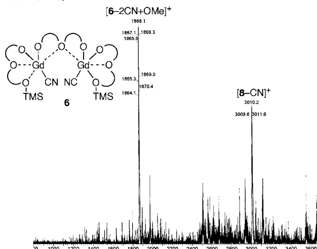
(A) \text{Gd}(\text{O}^i\text{Pr})_3 + \mathbf{5} + \text{TMSCN} (1:2:10)
